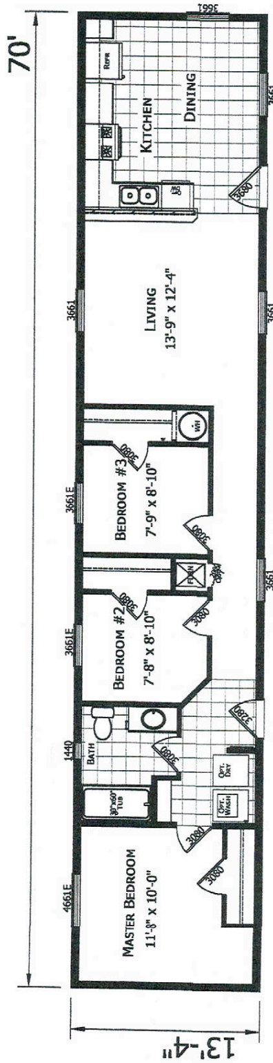
MODEL 122-07-F-27025 3 BEDROOM 1 BATH 70'-0" x 13'-4" 933 SQ. FT. TOTAL 06-18-21
