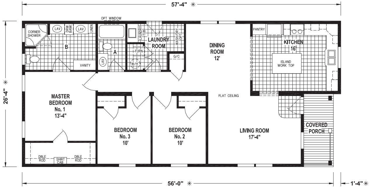
M932/57-428 (1,422 SQ. FT.) 3BEDROOM - 2BATHS
